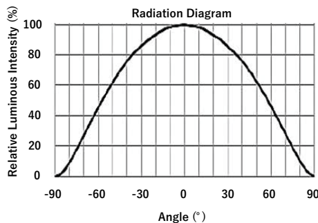
Radiation Characteristic
